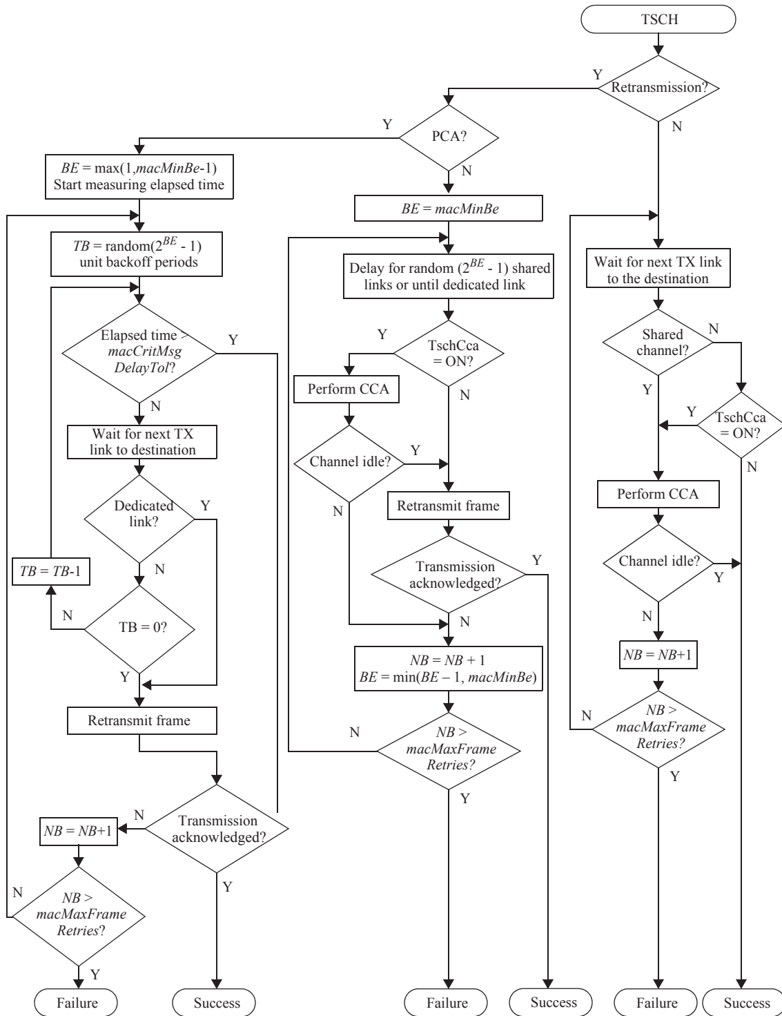
Figure 6-6—TSCH Retransmission backoff algorithm
