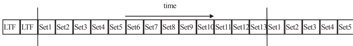
Figure 21-10—Pilot tone sets for Option 1
